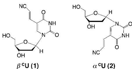
Figure 2. Structures of \beta -5-cyanovinyldeoxyuridine ( \beta^5\text{CUp} ) and \alpha -5-cyanovinyldeoxyuridine ( \alpha^5\text{CU} ).
