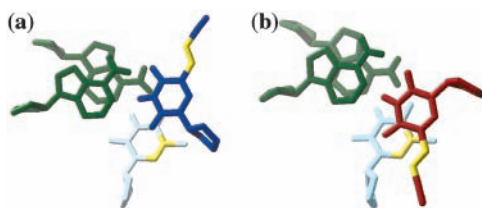
Figure 3. Molecular modeling of the stacking geometry in B-form DNA. The model was optimized by AMBER* force field in water using MacroModel version 8.1. Blue, red, green, and water blue molecules are \beta^5\text{CUp} , \alpha^5\text{CU} , dA, and dT, respectively. The vinyl group and C5–C6 double bond of the 5'-terminal dT are shown in yellow: (a) 3'-terminal \beta^5\text{CUp} and 5'-terminal dT, (b) 3'-terminal \alpha^5\text{CU} and 5'-terminal dT.
